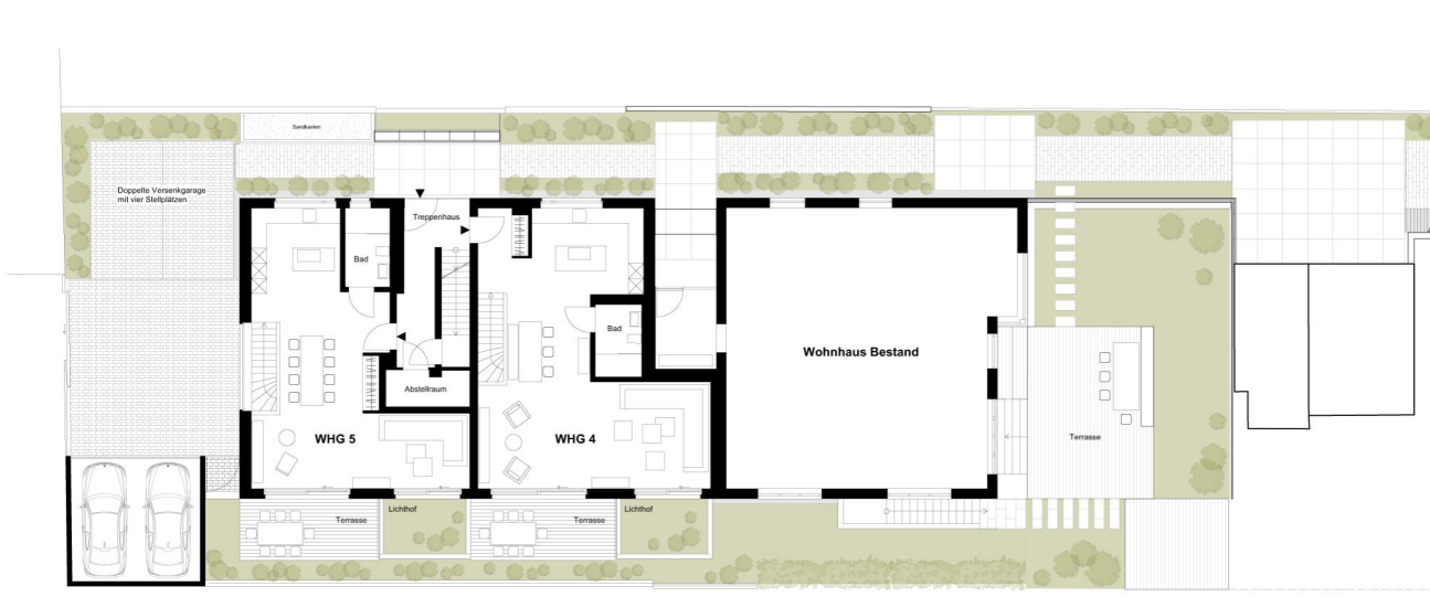
Grundriss Erdgeschoss © tools off.architecture
